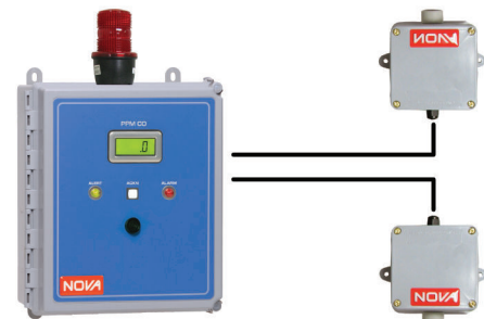
580DR2 - Alarm Unit and Dual Diffusion-Style Sensors in Separate Enclosures
